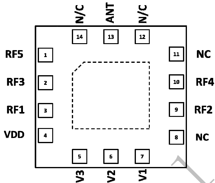
Fig. 2 D7005 Pin Layout (Top View)
